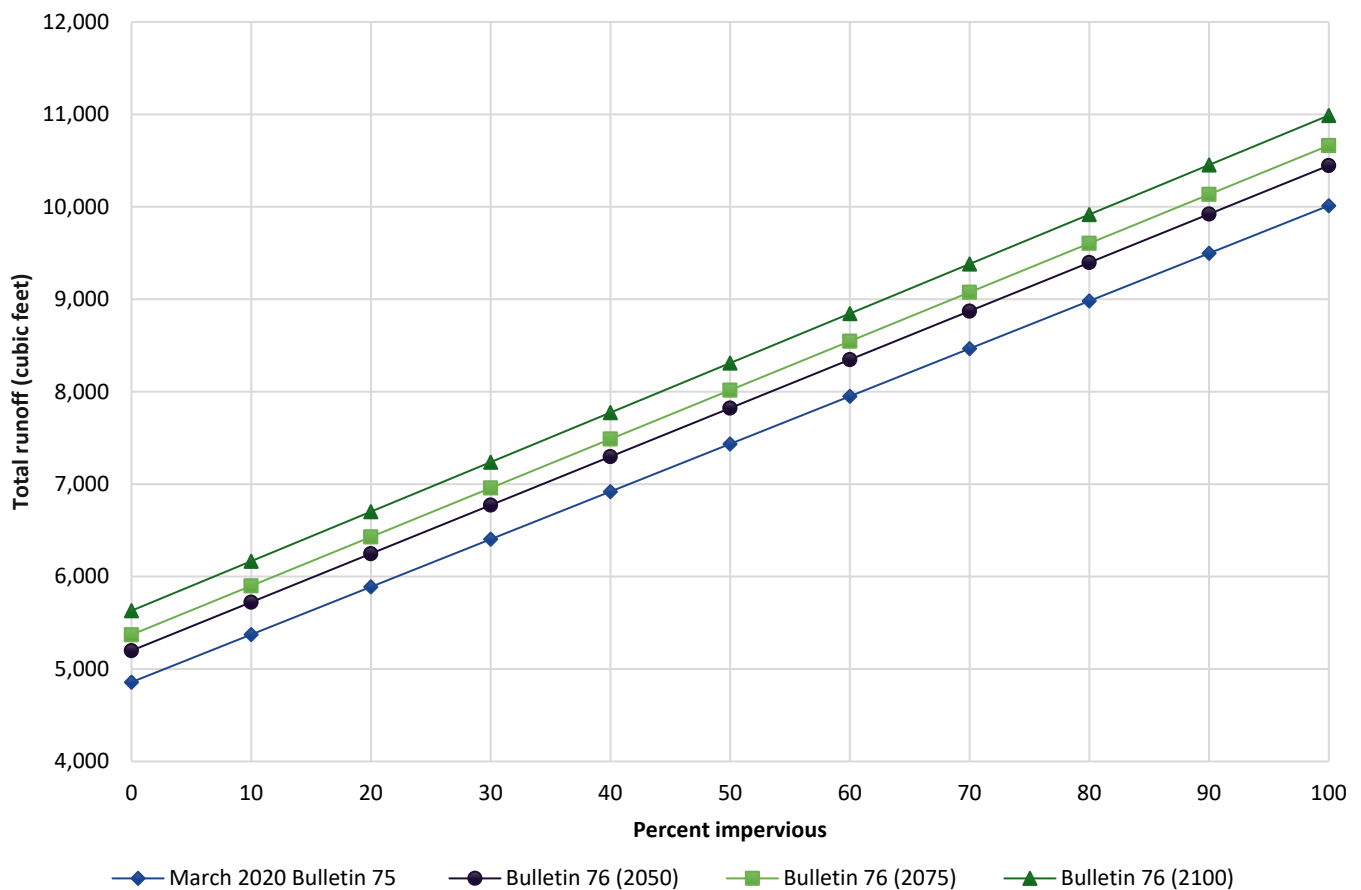
Figure 11: Total runoff for 1-acre during 10-year, 2-hour event with different percent impervious scenarios
